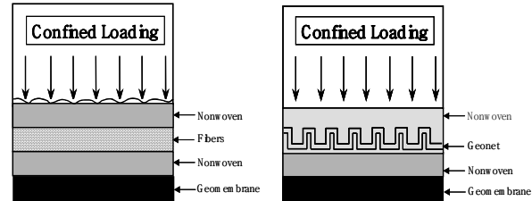
Figure 3. Schematic diagram of intrusion for smart geotextiles and geonet composites under confined loading
